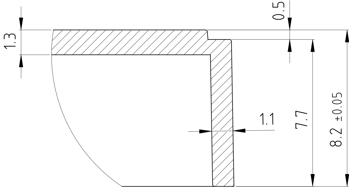
DETAIL C SCALE 10 : 1
