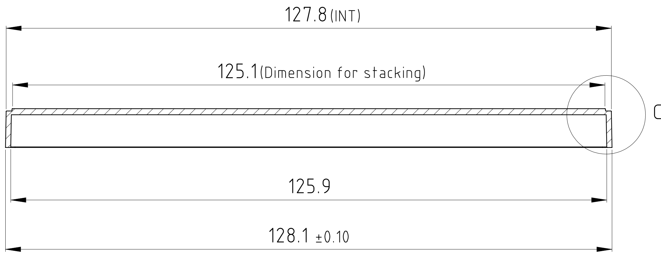
SECTION B-B
